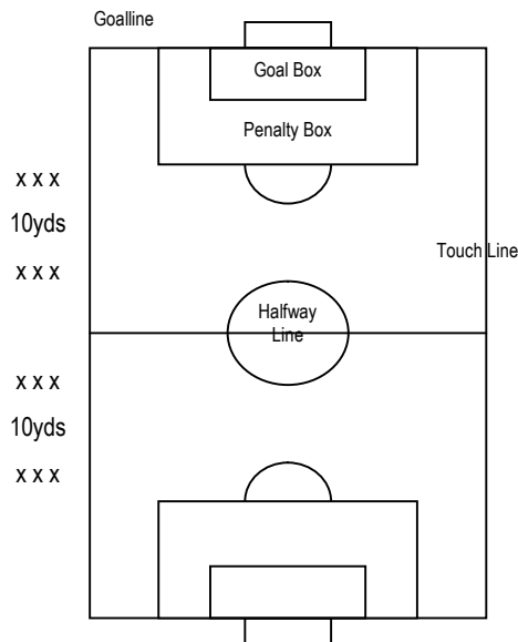
Substitution Diagram
